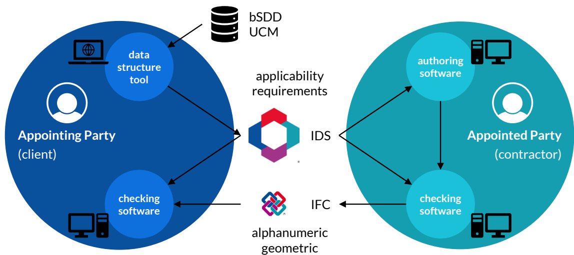
Abb. 3.52: IDS-Workflow
